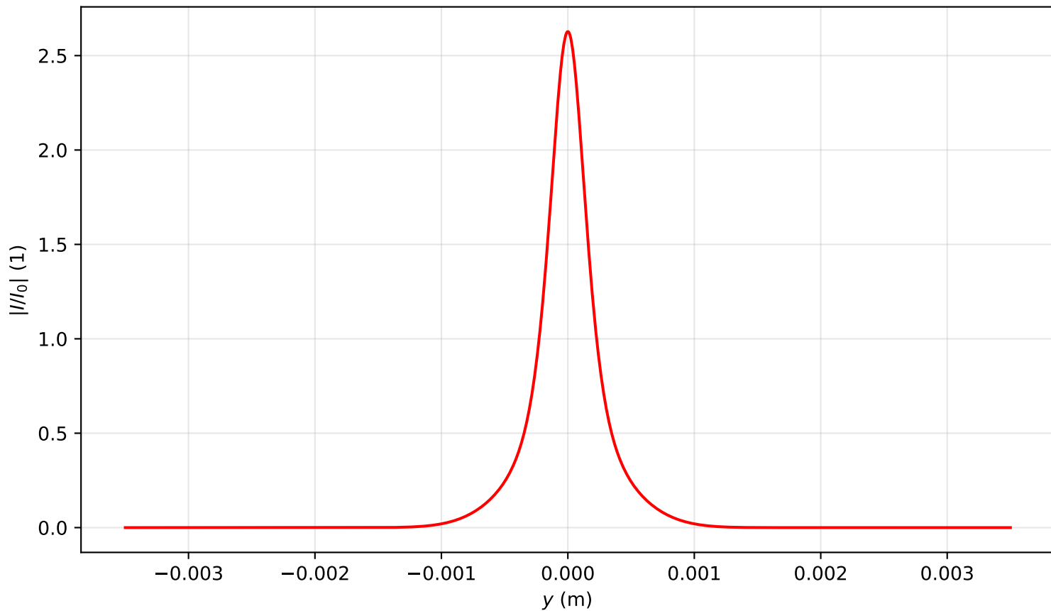
Intensity profile I(x=0, y, z=0.716)/I_0 , P_{in}=2.0P_{cr} , artificial time
